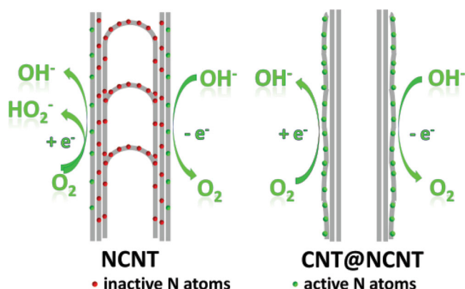
Figure 1. Scheme for the full exposure of 'active sites' on the surface: NCNTs with bulk doping of nitrogen atoms, while CNT@NCNT coaxial nanocables with surface enriched nitrogen for OER and ORR.
