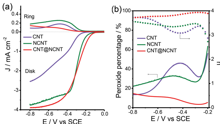
Figure 3. (a) Rotating ring disk voltammograms recorded for CNT, NCNT, and CNT@NCNT electrode in an \text{O}_2 -saturated 0.1 \text{ mol L}^{-1} KOH solution at a scan rate of 5.0 \text{ mV s}^{-1} . The disk current densities (bottom) and the corresponding ring current densities (top) are displayed separately as illustrated in the figure and the rotating speed of the electrode was 1600 \text{ rpm} . (b) Percentage of peroxide (solid line) and the electron transfer number ( n , dotted line) of the CNT, NCNT, and CNT@NCNT catalysts at various potentials, based on the corresponding RRDE data in (a).
