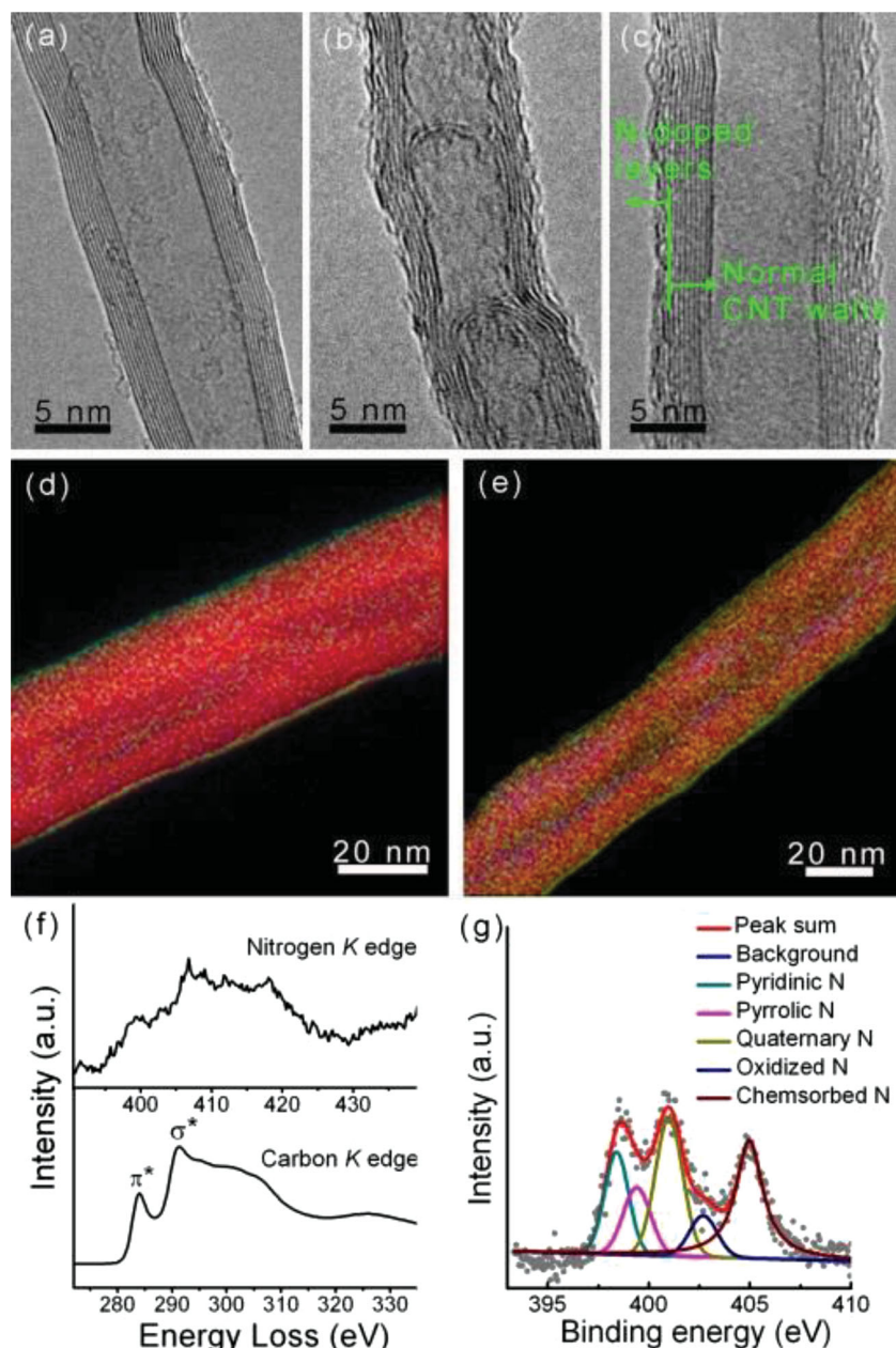
Figure 2. Structure of CNT@NCNT electrocatalyst with surface enriched nitrogen: TEM images of (a) pristine CNTs, (b) NCNTs, and (c) CNT@NCNT coaxial nanocables; the element mapping showing the distribution of N (green), C (red), and O (blue), of CNT@NCNT coaxial nanocables with the surface N/C ratio of (d) 0.0238 and (e) 0.0809; (f) high resolution EELS spectra of carbon K edge and nitrogen K edge and (g) N 1s core level XPS spectra for CNT@NCNT.
