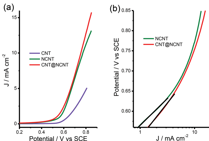
Figure 4. (a) OER currents of the CNT, NCNT, and CNT@NCNT catalysts in 0.1 \text{ mol L}^{-1} KOH solution at a scan rate of 5.0 \text{ mV s}^{-1} . (b) Tafel plots of OER currents for NCNT and CNT@NCNT in (a).
